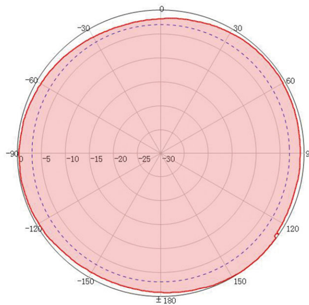
Axial Ratio
