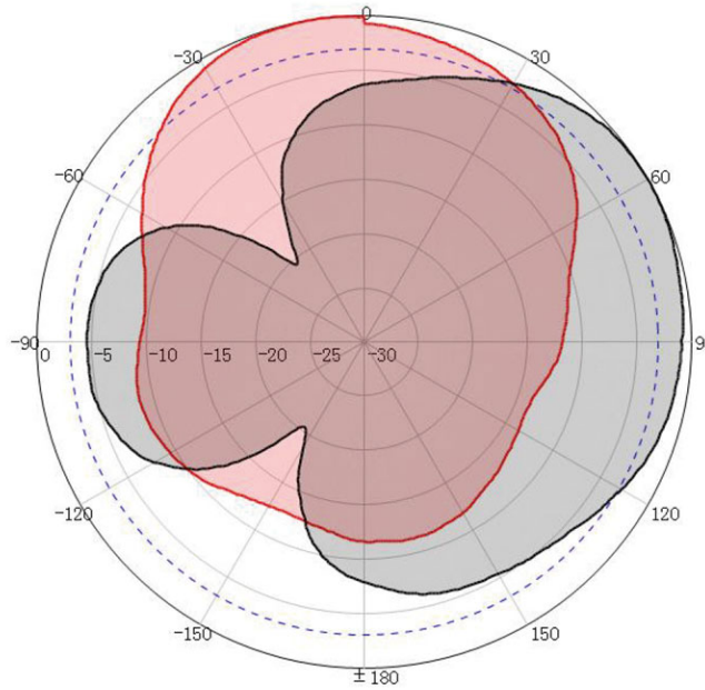
915MHz
